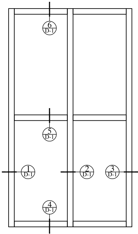
CW250P, 2 1/2" X 5 1/2" CURTAIN WALL WITH POLYAMIDE PRESSURE BAR 1" GLAZING SETUP
