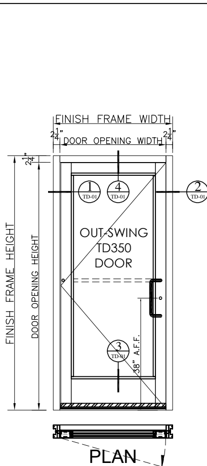
ALUMINUM STOREFRONT ELEVATIONS SCALE: 3/8" = 1'-0"
