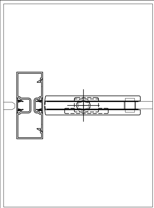
D PATCH FITTING / JAMB
