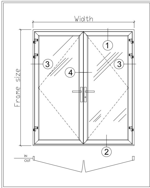
BD-325 SERIES BALCONY DOOR SWING - OUT PAIR DOOR
