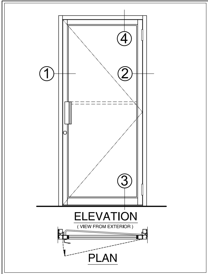
NARROW STILE DOOR (D200 SERIES) STANDARD HANDLE - 1/4" GLAZING
