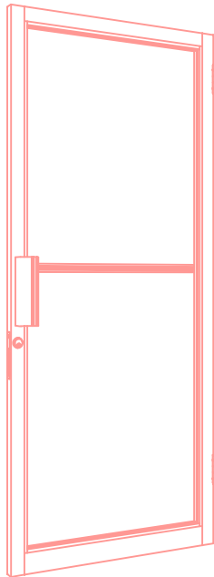
Standard D200 Narrow Stile 2 1/8" Stile & Top Rail 3 1/8" Bottom Rail
