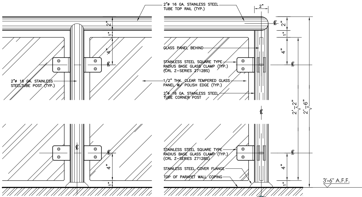
GLASS RAILING TYPICAL ELEVATION
