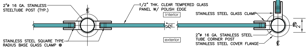
GLASS RAILING TYPICAL PLAN
