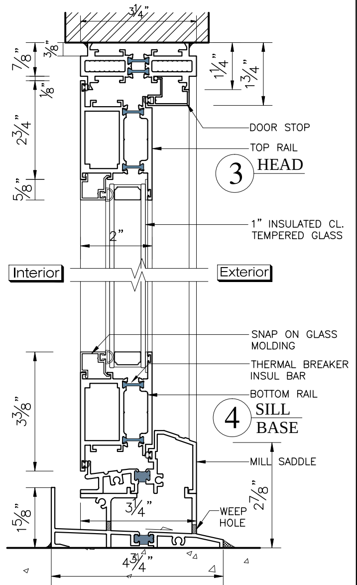
BD-325 SERIES BALCONY DOOR (OPEN INWARD)
