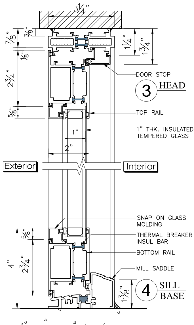
BD-325 SERIES BALCONY PAIR DOOR (OPEN OUTWARD)
