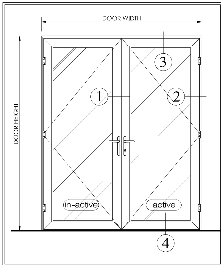
BD-325 SERIES BALCONY PAIR DOOR (OPEN OUTWARD)
