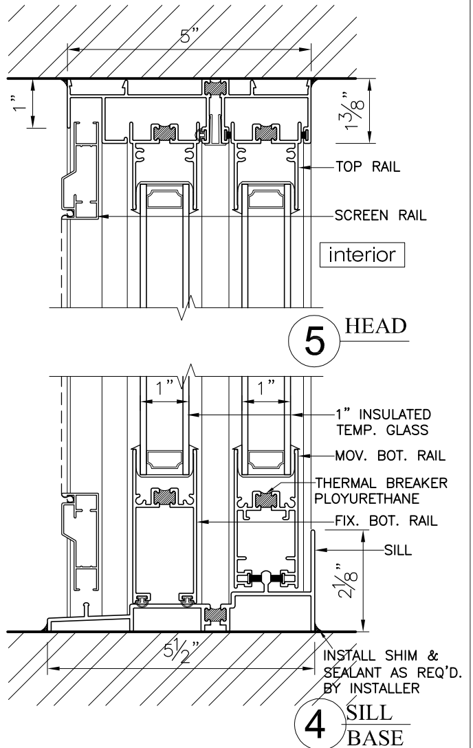
PD-2000 SERIES PATIO SLIDING DOOR
